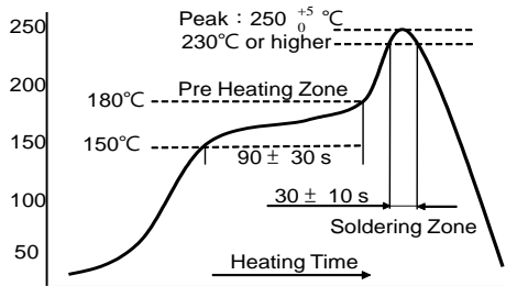
Reflow Soldering
